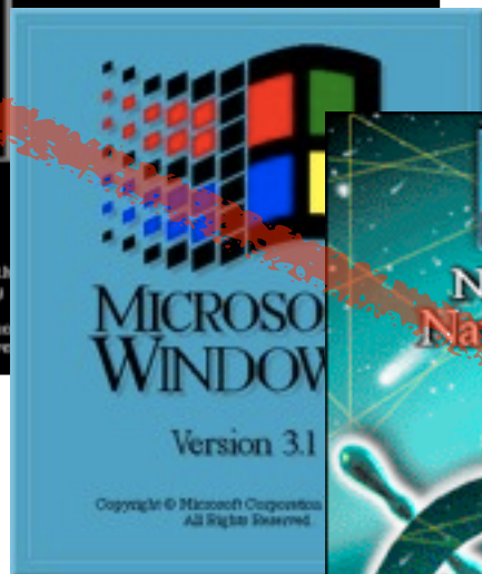
Windows
